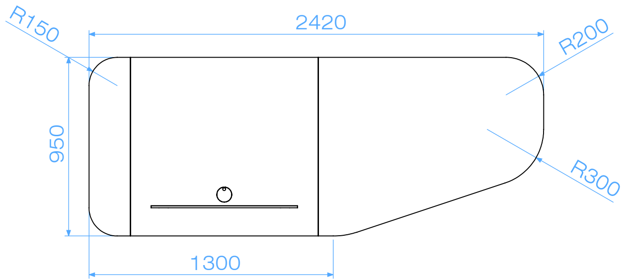
PLAN VIEW
