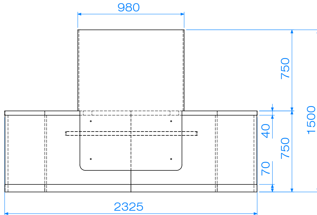
FRONT ELEVATION
